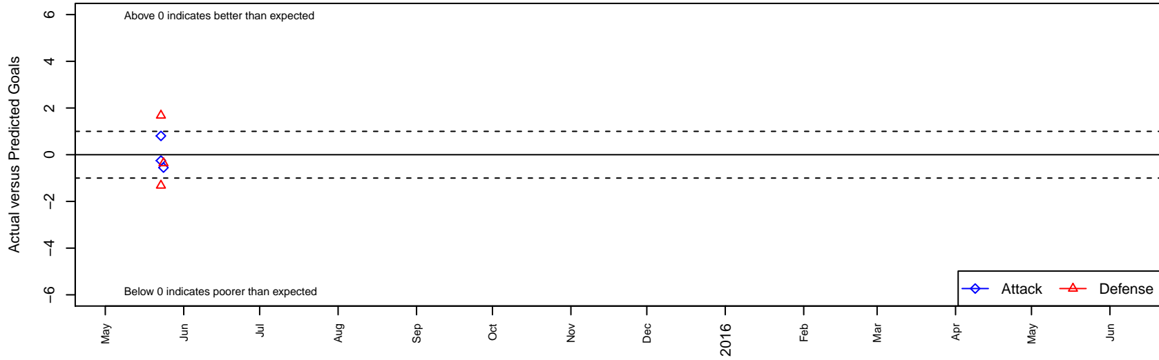
Southwestern YSC LA Hawks B03 Dots are actual minus expected GF (blue circles) and GA (red triangles). Blue line is smoothed change in attack strength. Red is smoothed change in defense strength.
